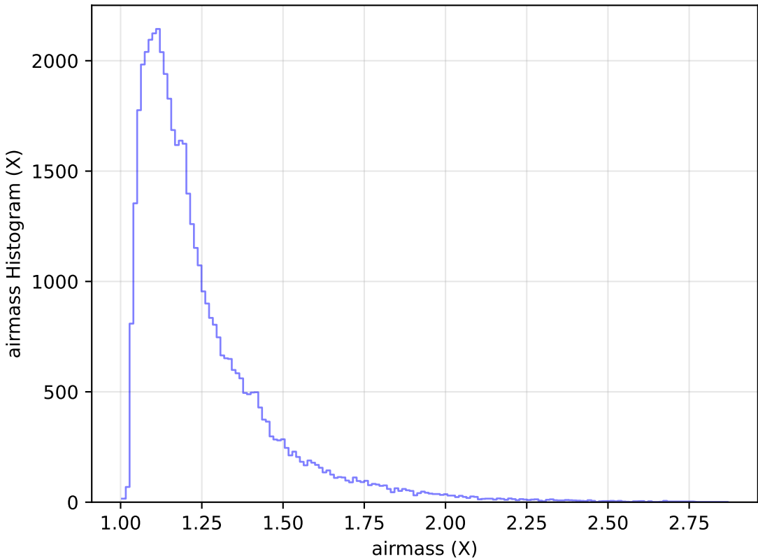
too_elab_r64_d2_ugrizy_v3.4_10yrs Yr 1 y band: airmass Histogram
