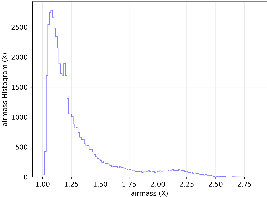
too_elab_r64_d2_ugrizy_v3.4_10yrs Yr 1 r band: airmass Histogram
