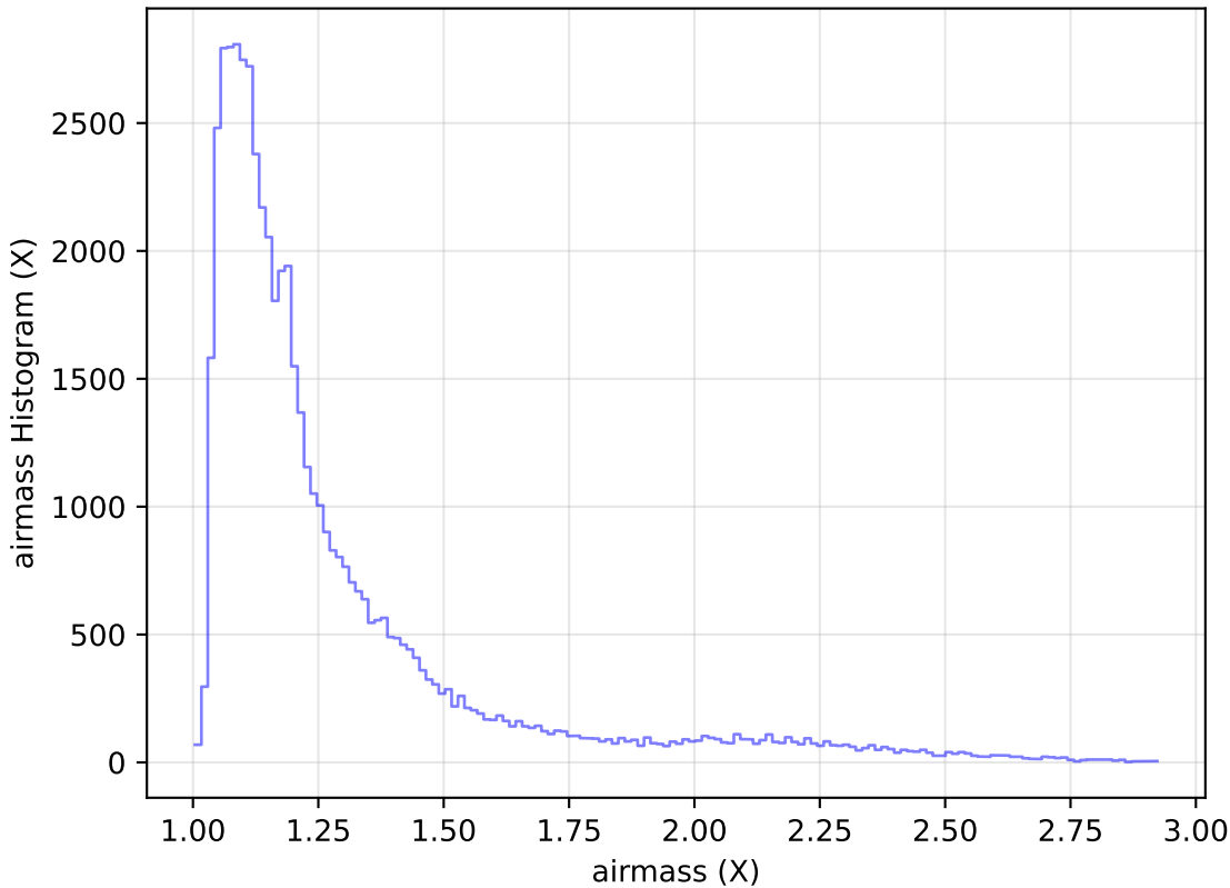
too_elab_r64_d2_ugrizy_v3.4_10yrs Yr 1 i band: airmass Histogram
