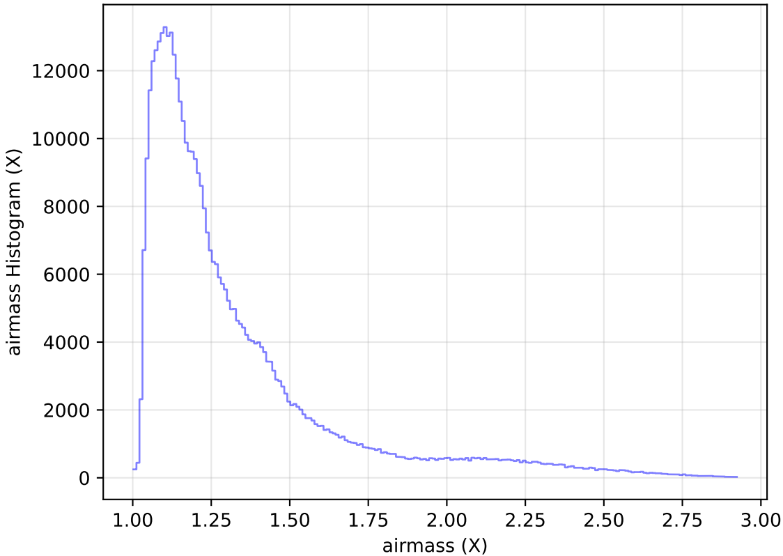
too_elab_r64_d2_ugrizy_v3.4_10yrs WFD z band: airmass Histogram
