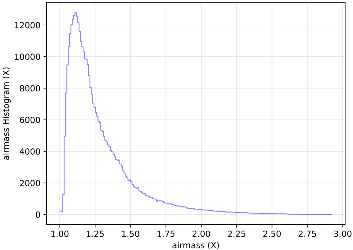
too_elab_r64_d2_ugrizy_v3.4_10yrs WFD y band: airmass Histogram
