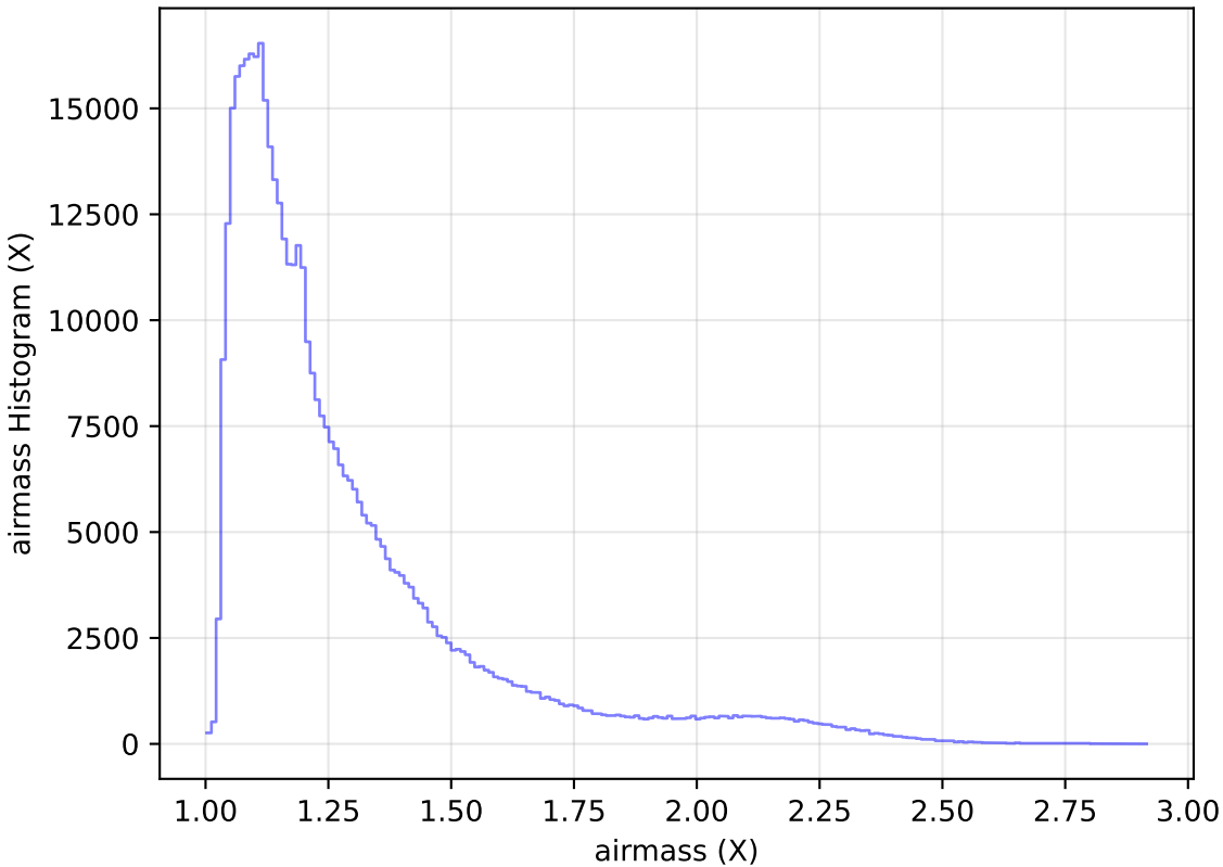
too_elab_r64_d2_ugrizy_v3.4_10yrs WFD r band: airmass Histogram
