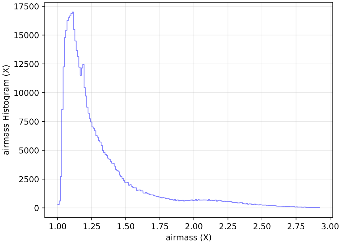
too_elab_r64_d2_ugrizy_v3.4_10yrs WFD i band: airmass Histogram
