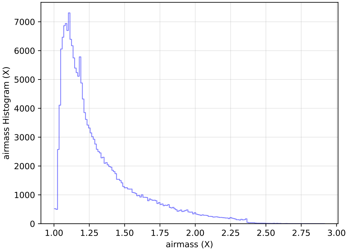
too_elab_r64_d2_ugrizy_v3.4_10yrs WFD g band: airmass Histogram
