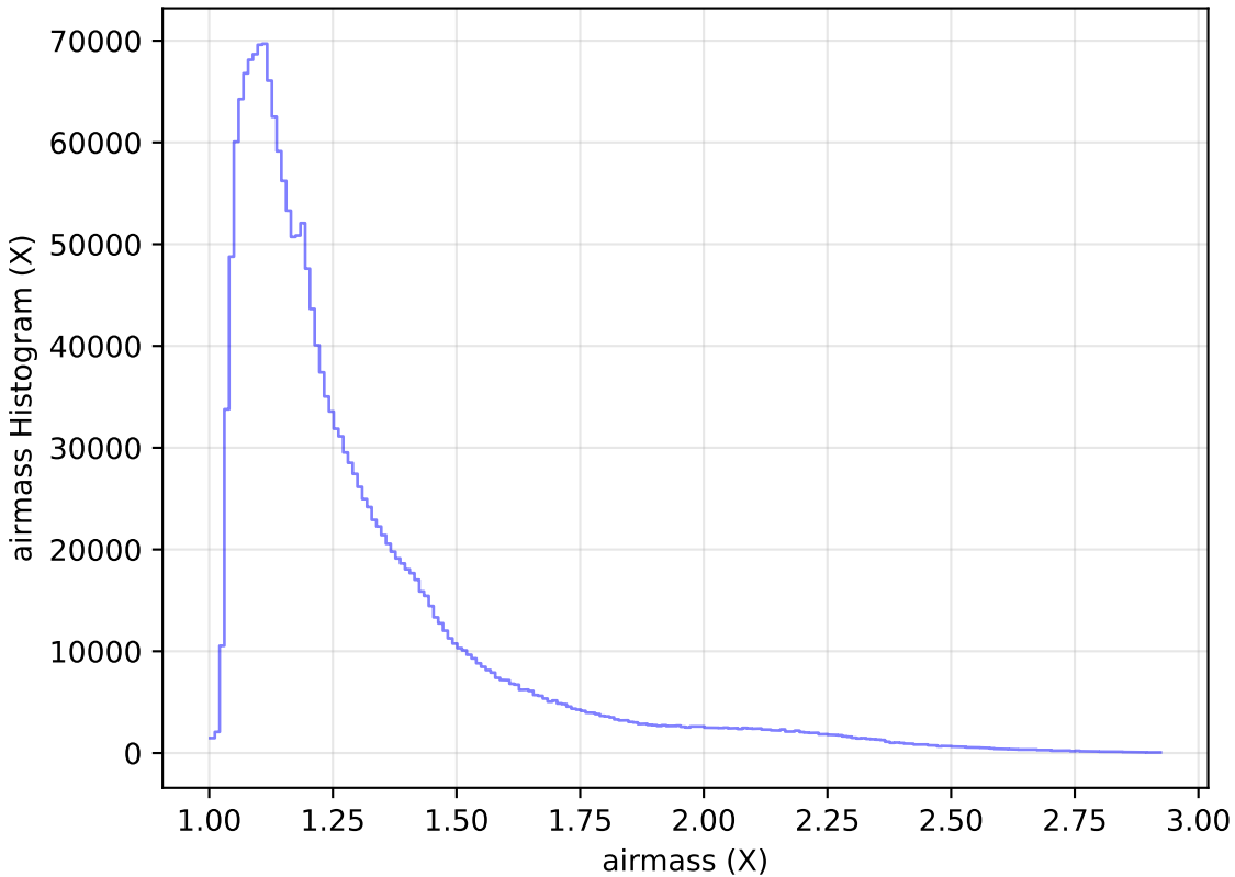
too_elab_r64_d2_ugrizy_v3.4_10yrs WFD all bands: airmass Histogram
