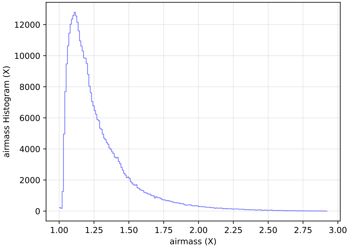
too_elab_r64_d2_ugrizy_v3.4_10yrs All sky y band: airmass Histogram
