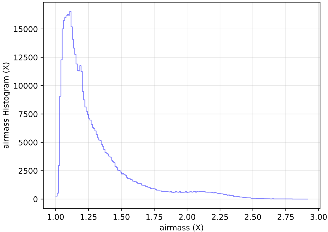
too_elab_r64_d2_ugrizy_v3.4_10yrs All sky r band: airmass Histogram
