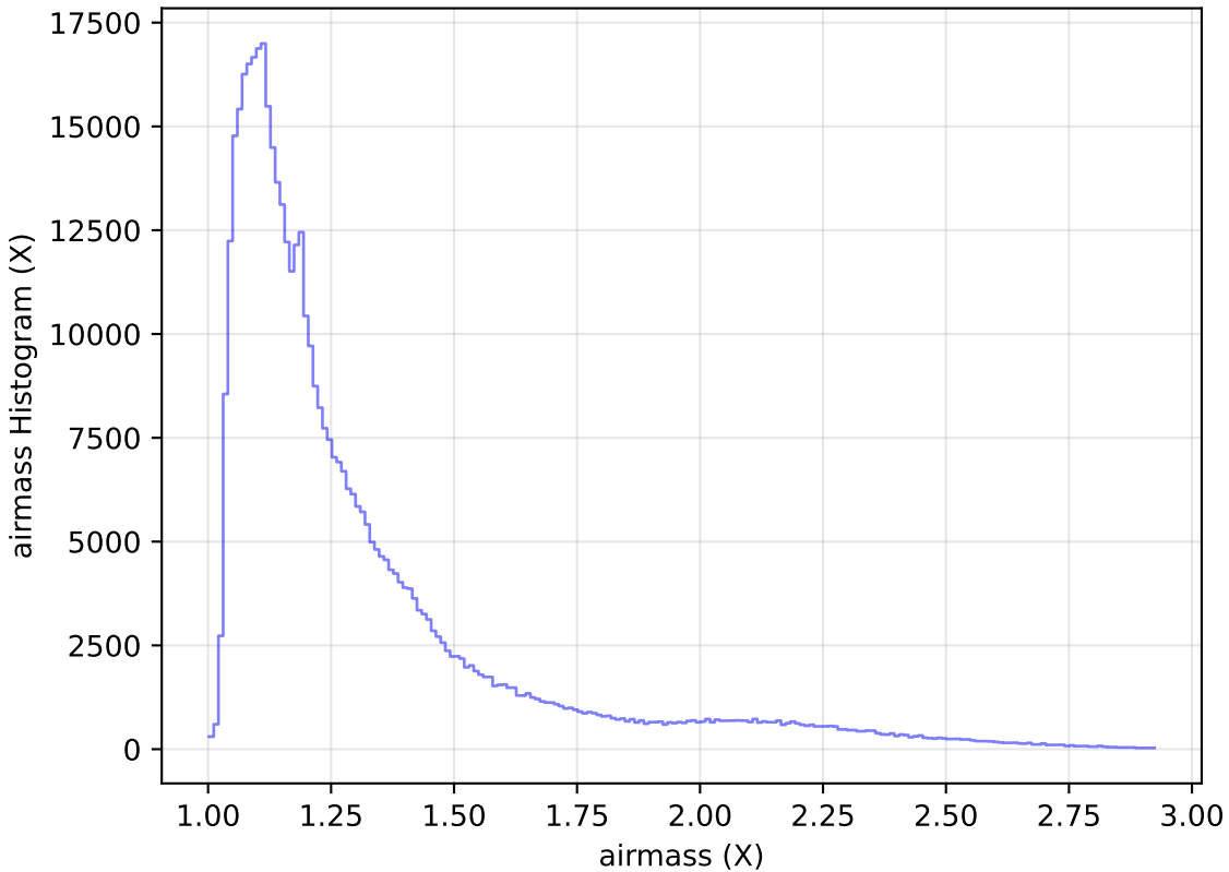
too_elab_r64_d2_ugrizy_v3.4_10yrs All sky i band: airmass Histogram
