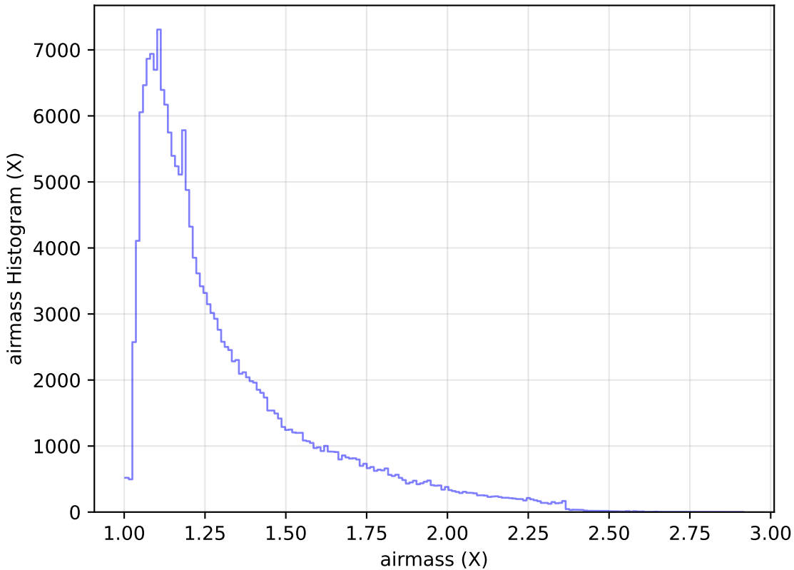
too_elab_r64_d2_ugrizy_v3.4_10yrs All sky g band: airmass Histogram
