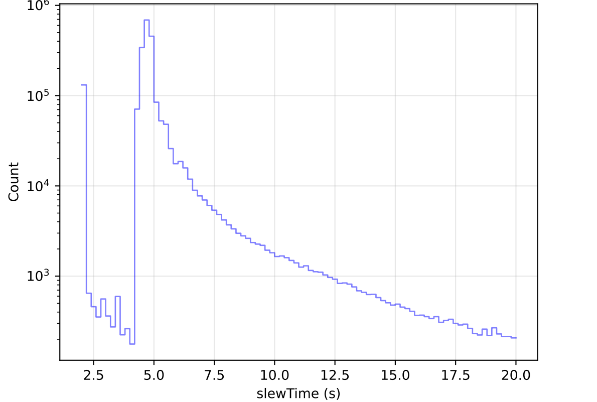
too_elab_r64_d2_ugrizy_v3.4_10yrs All visits: Zoom Slew Time Histogram
