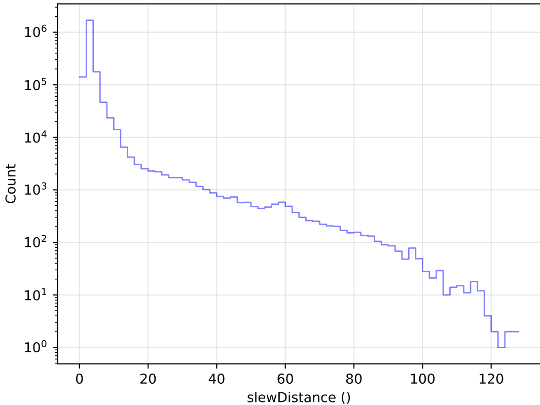
too_elab_r64_d2_ugrizy_v3.4_10yrs All visits: Slew Distance Histogram
