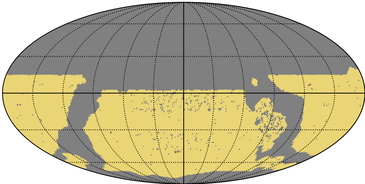
too_elab_r64_d2_ugrizy_v3.4_10yrs WFD: RapidRevisits
