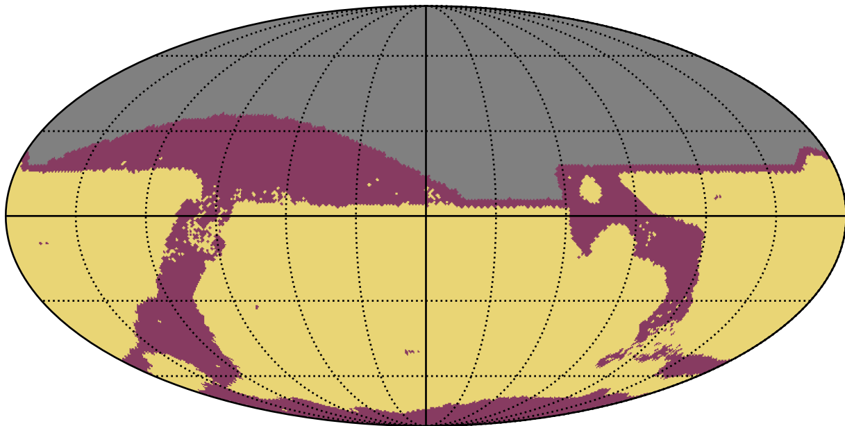
too_elab_r64_d2_ugrizy_v3.4_10yrs All sky: RapidRevisits
