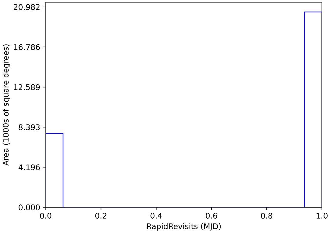
too_elab_r64_d2_ugrizy_v3.4_10yrs All sky: RapidRevisits
