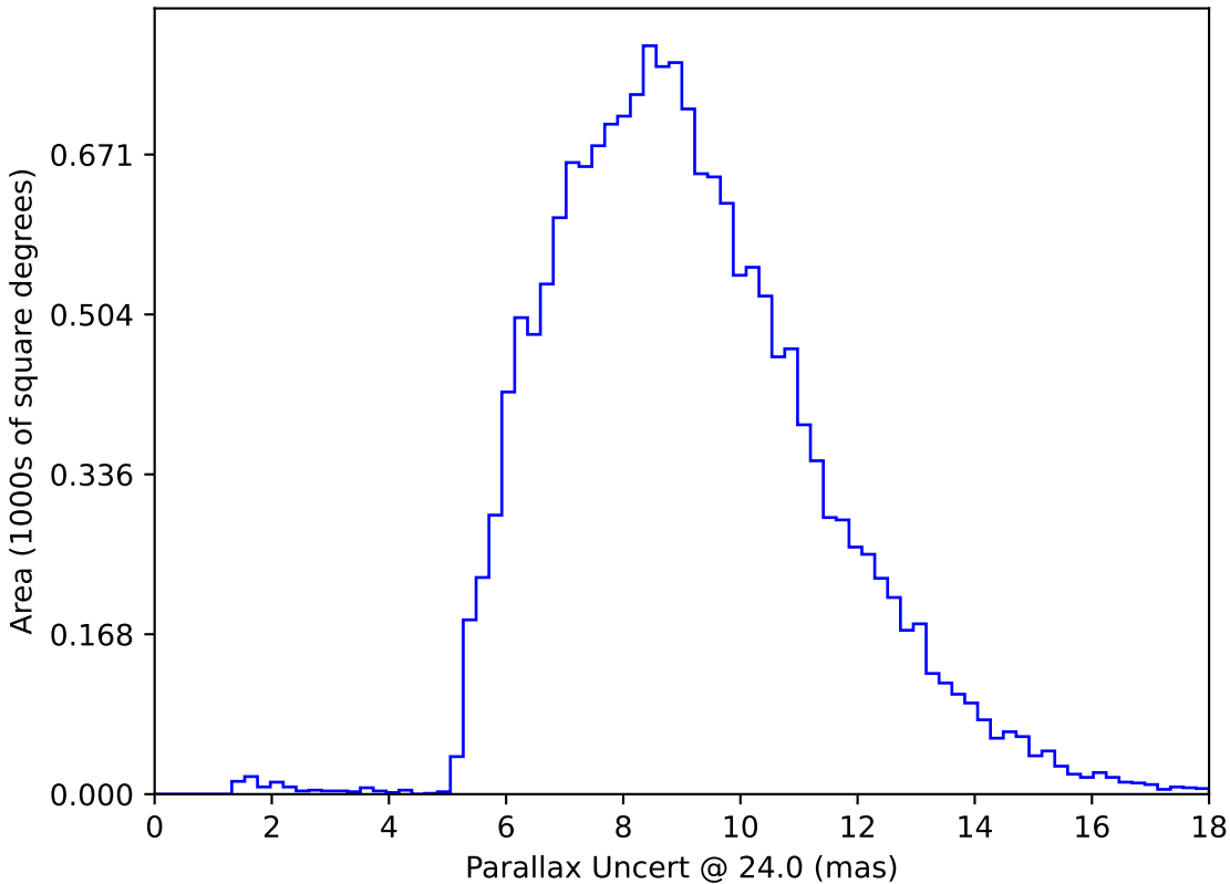
too_elab_r64_d2_ugrizy_v3.4_10yrs WFD: Parallax Uncert @ 24.0
