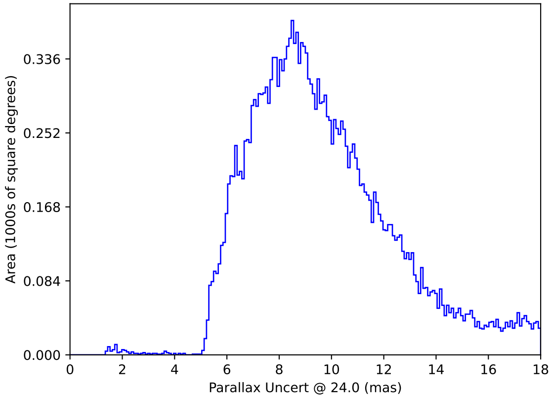
too_elab_r64_d2_ugrizy_v3.4_10yrs All sky: Parallax Uncert @ 24.0
