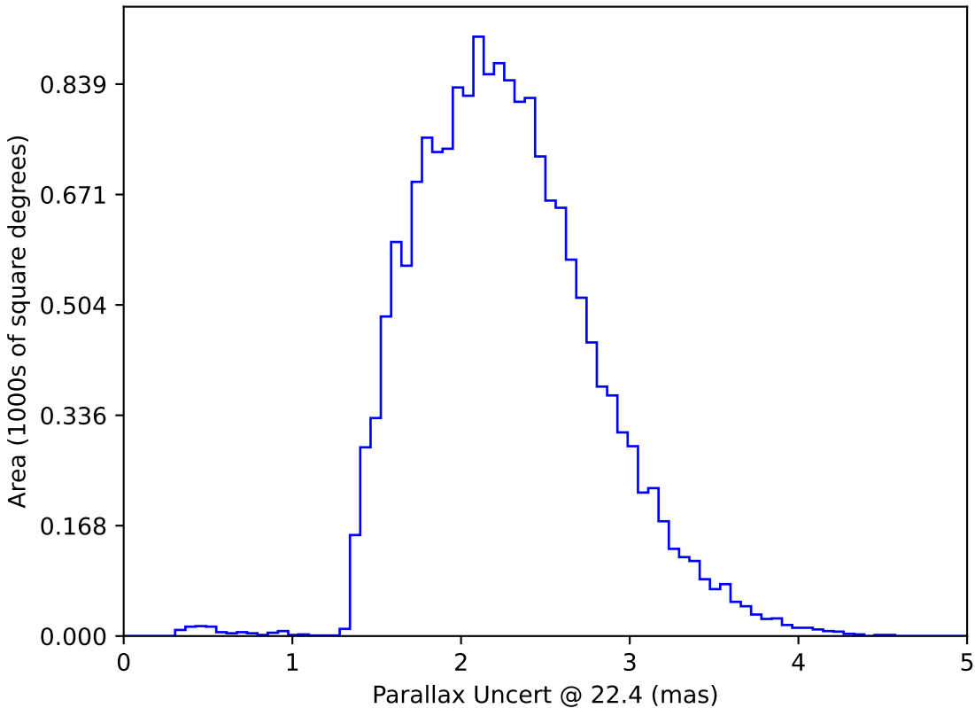
too_elab_r64_d2_ugrizy_v3.4_10yrs WFD: Parallax Uncert @ 22.4
