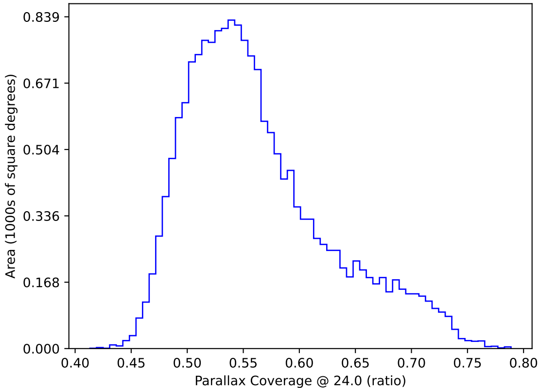
too_elab_r64_d2_ugrizy_v3.4_10yrs WFD: Parallax Coverage @ 24.0
