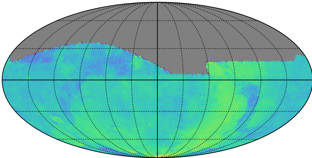
too_elab_r64_d2_ugrizy_v3.4_10yrs All sky: Parallax Coverage @ 24.0
