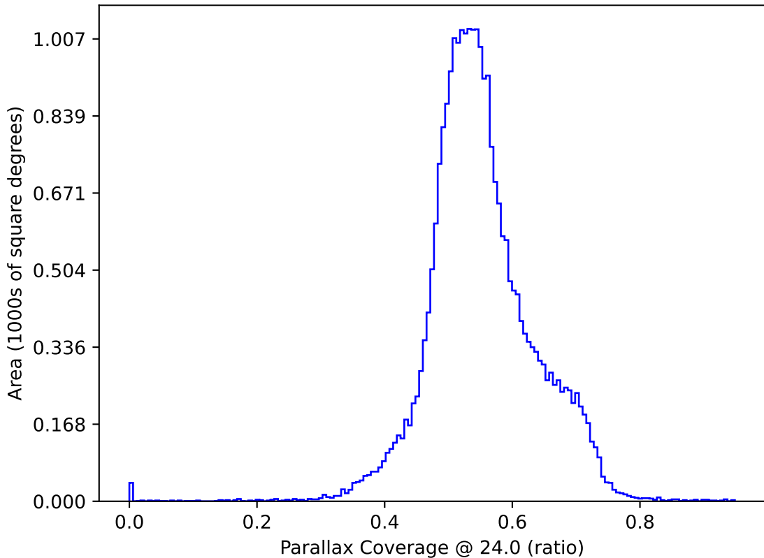
too_elab_r64_d2_ugrizy_v3.4_10yrs All sky: Parallax Coverage @ 24.0
