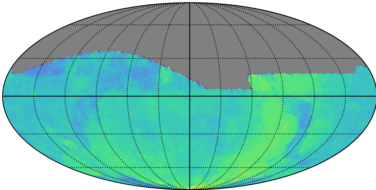
too_elab_r64_d2_ugrizy_v3.4_10yrs All sky: Parallax Coverage @ 22.4
