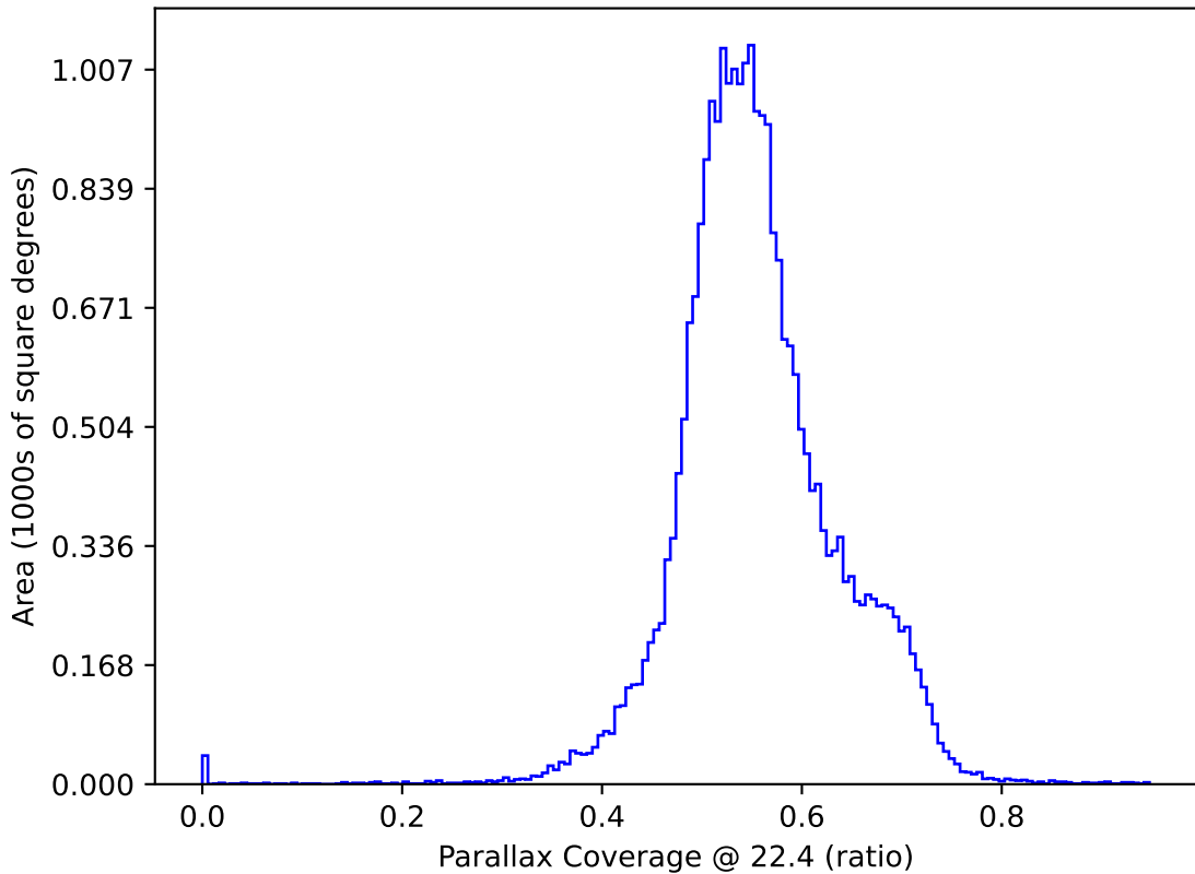
too_elab_r64_d2_ugrizy_v3.4_10yrs All sky: Parallax Coverage @ 22.4
