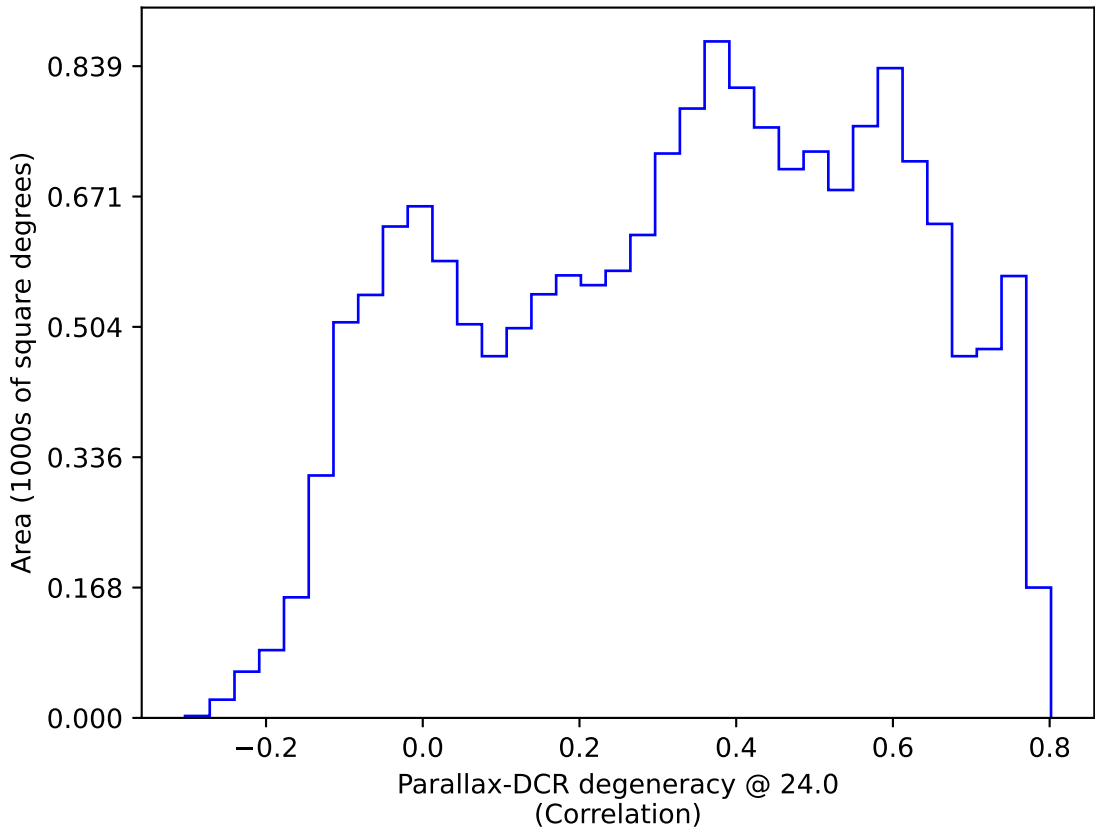
too_elab_r64_d2_ugrizy_v3.4_10yrs WFD: Parallax-DCR degeneracy @ 24.0
