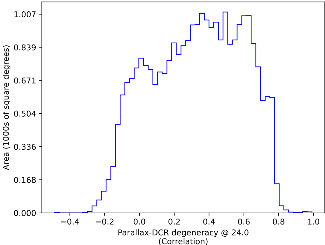
too_elab_r64_d2_ugrizy_v3.4_10yrs All sky: Parallax-DCR degeneracy @ 24.0
