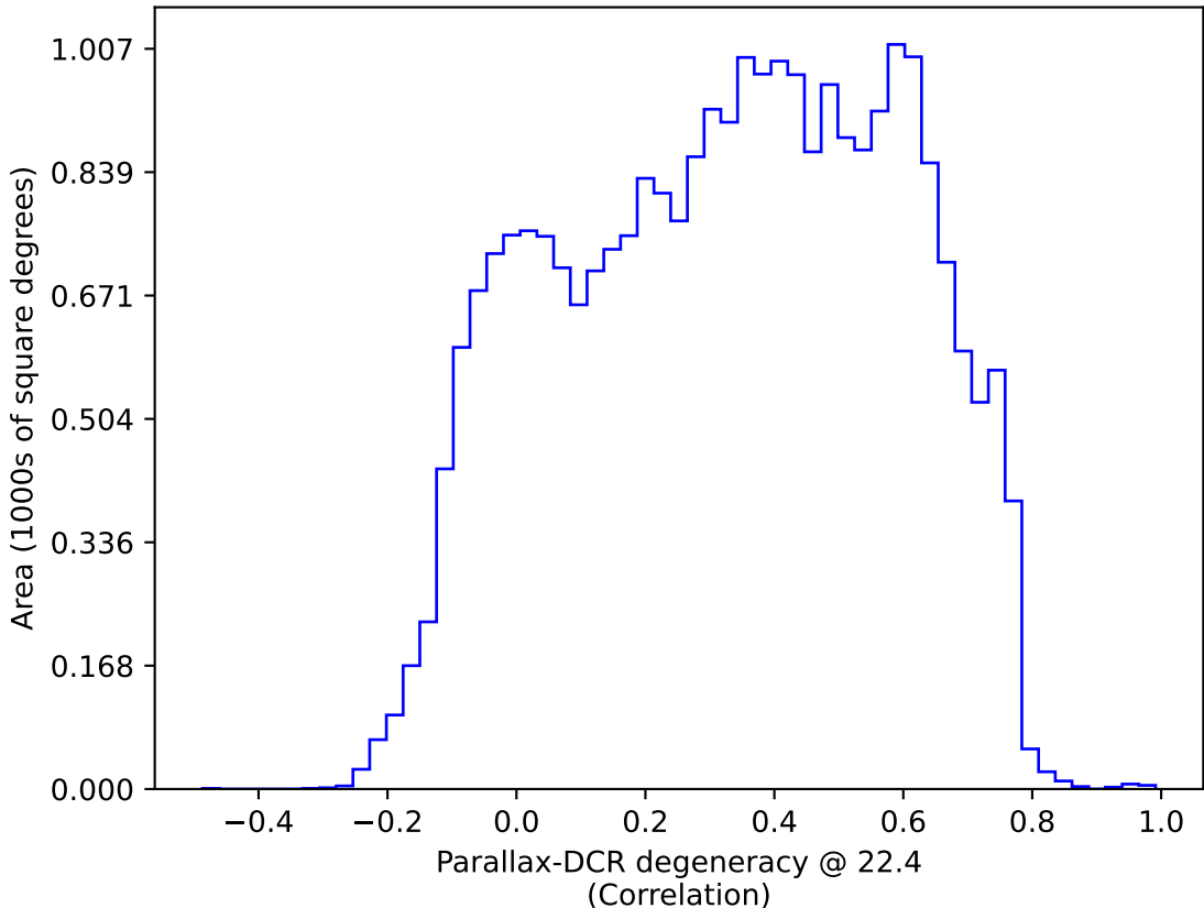
too_elab_r64_d2_ugrizy_v3.4_10yrs All sky: Parallax-DCR degeneracy @ 22.4
