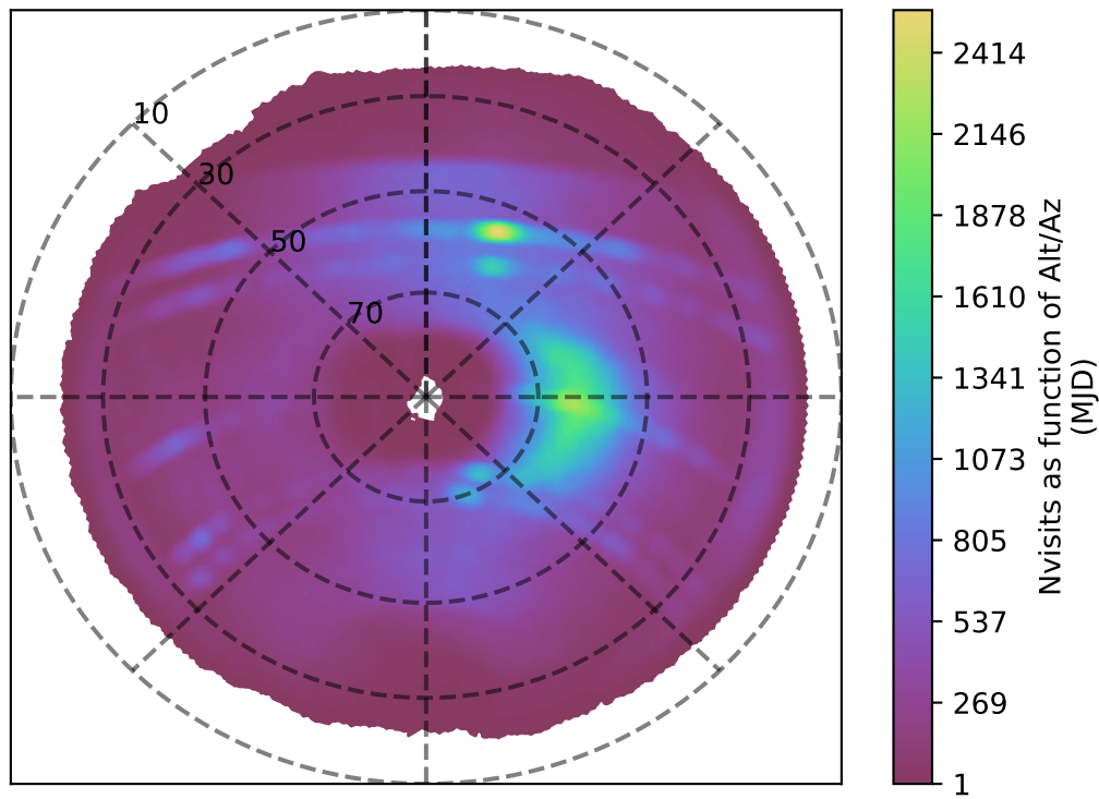
too_elab_r64_d2_ugrizy_v3.4_10yrs z band: Nvisits as function of Alt/Az
