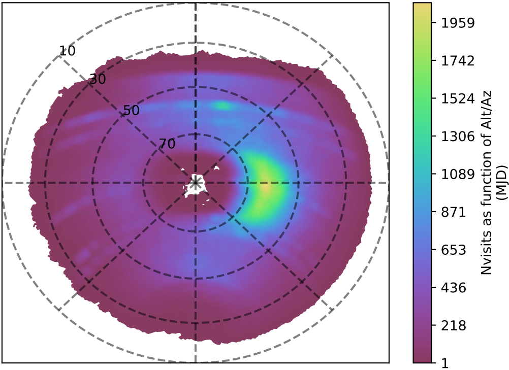
too_elab_r64_d2_ugrizy_v3.4_10yrs y band: Nvisits as function of Alt/Az
