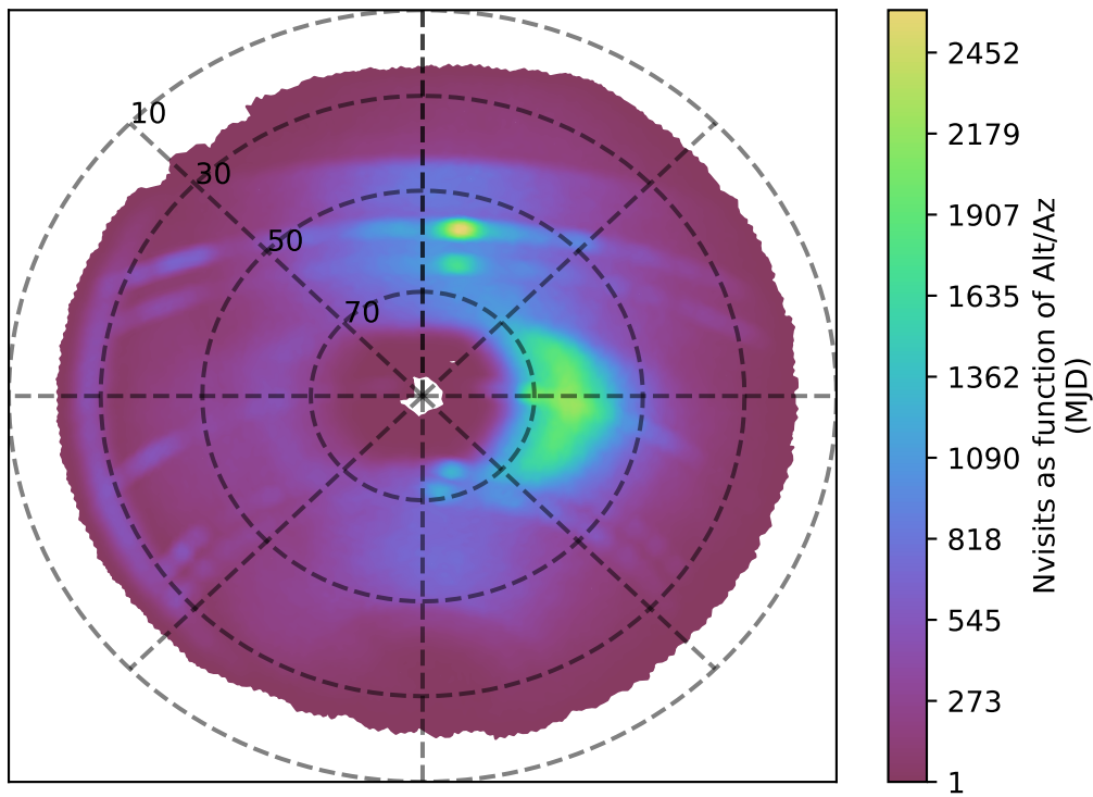
too_elab_r64_d2_ugrizy_v3.4_10yrs r band: Nvisits as function of Alt/Az
