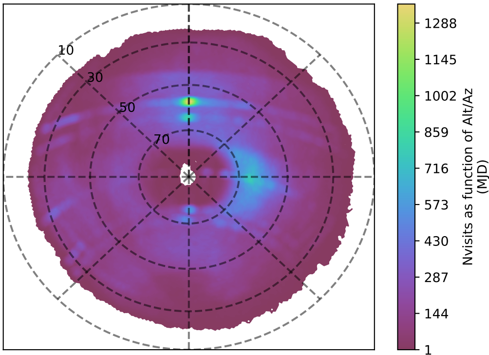
too_elab_r64_d2_ugrizy_v3.4_10yrs g band: Nvisits as function of Alt/Az
