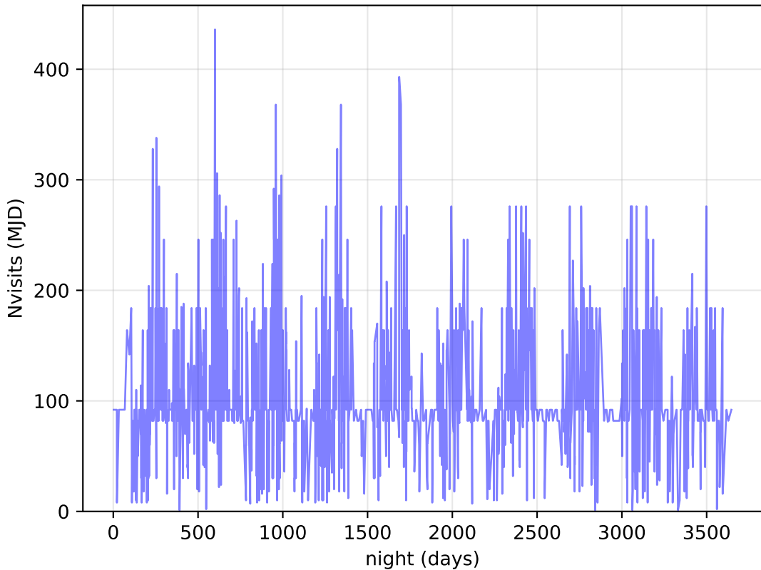
too_elab_r64_d2_ugrizy_v3.4_10yrs DDF: Nvisits
