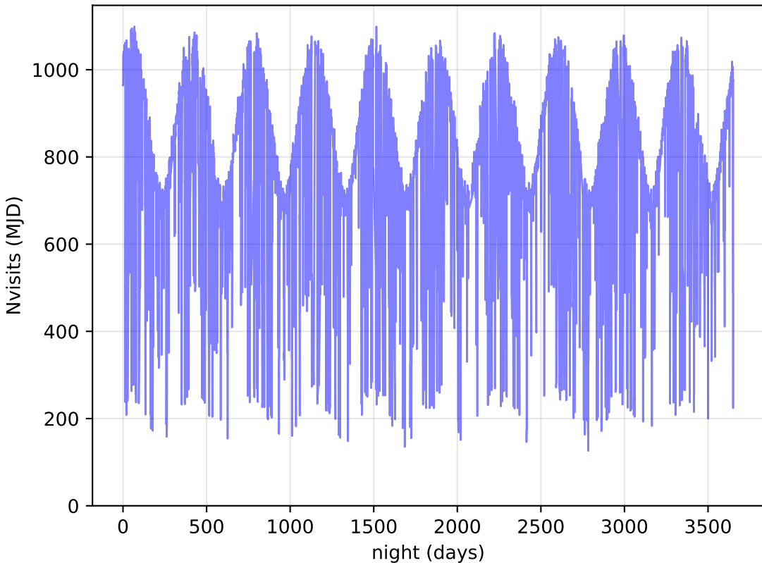
too_elab_r64_d2_ugrizy_v3.4_10yrs All visits: Nvisits
