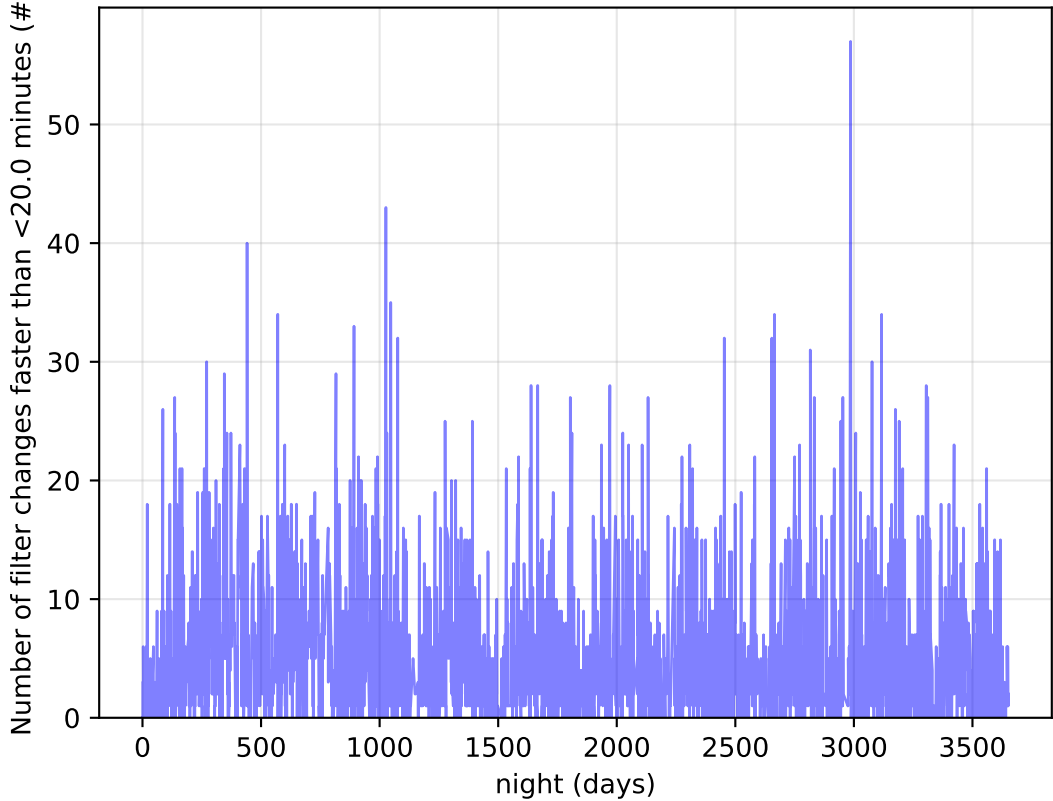
too_elab_r64_d2_ugrizy_v3.4_10yrs Per Night: Number of filter changes faster than <20.0 minutes
