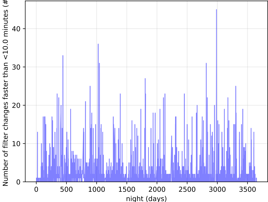
too_elab_r64_d2_ugrizy_v3.4_10yrs Per Night: Number of filter changes faster than <10.0 minutes
