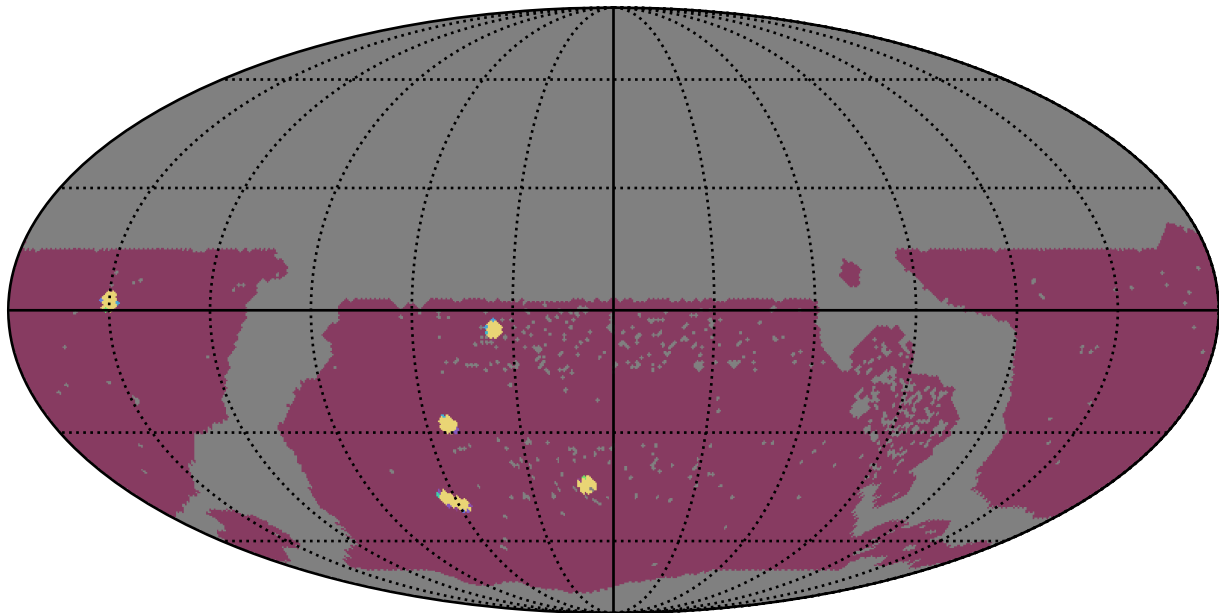
too_elab_r64_d2_ugrizy_v3.4_10yrs WFD: NumberOfQuickRevisits
