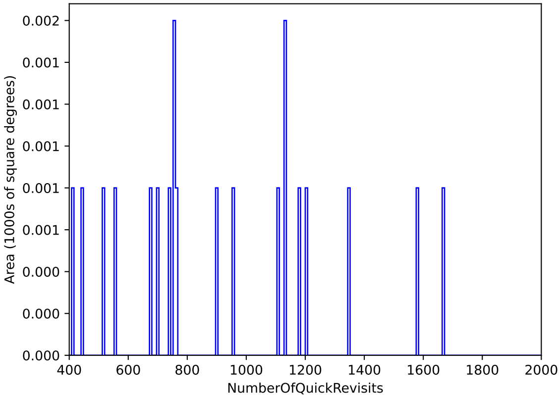
too_elab_r64_d2_ugrizy_v3.4_10yrs WFD: NumberOfQuickRevisits
