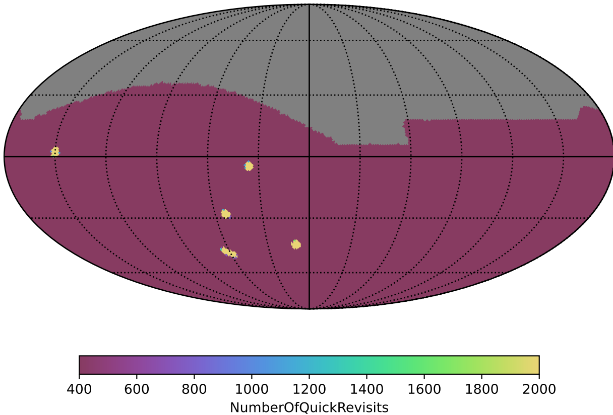
too_elab_r64_d2_ugrizy_v3.4_10yrs All sky: NumberOfQuickRevisits
