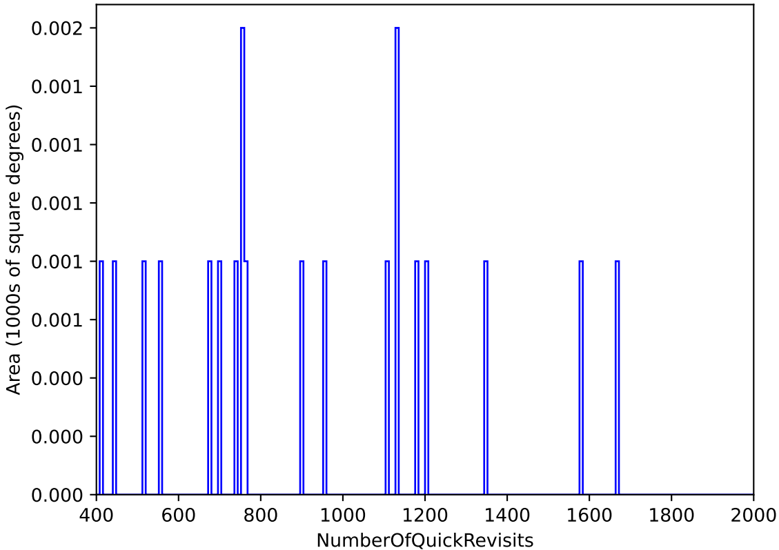
too_elab_r64_d2_ugrizy_v3.4_10yrs All sky: NumberOfQuickRevisits
