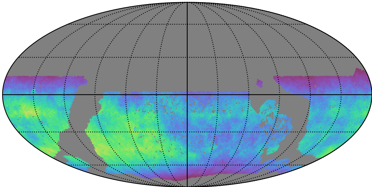
too_elab_r64_d2_ugrizy_v3.4_10yrs WFD z band: Normalized Teff
