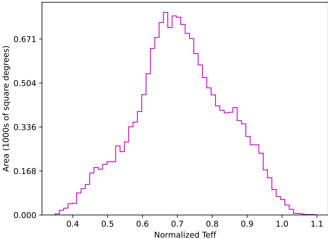
too_elab_r64_d2_ugrizy_v3.4_10yrs WFD z band: Normalized Teff
