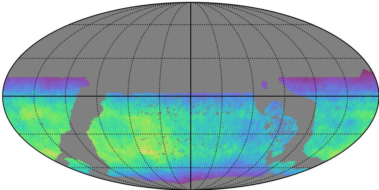
too_elab_r64_d2_ugrizy_v3.4_10yrs WFD y band: Normalized Teff
