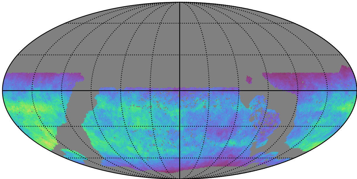
too_elab_r64_d2_ugrizy_v3.4_10yrs WFD u band: Normalized Teff
