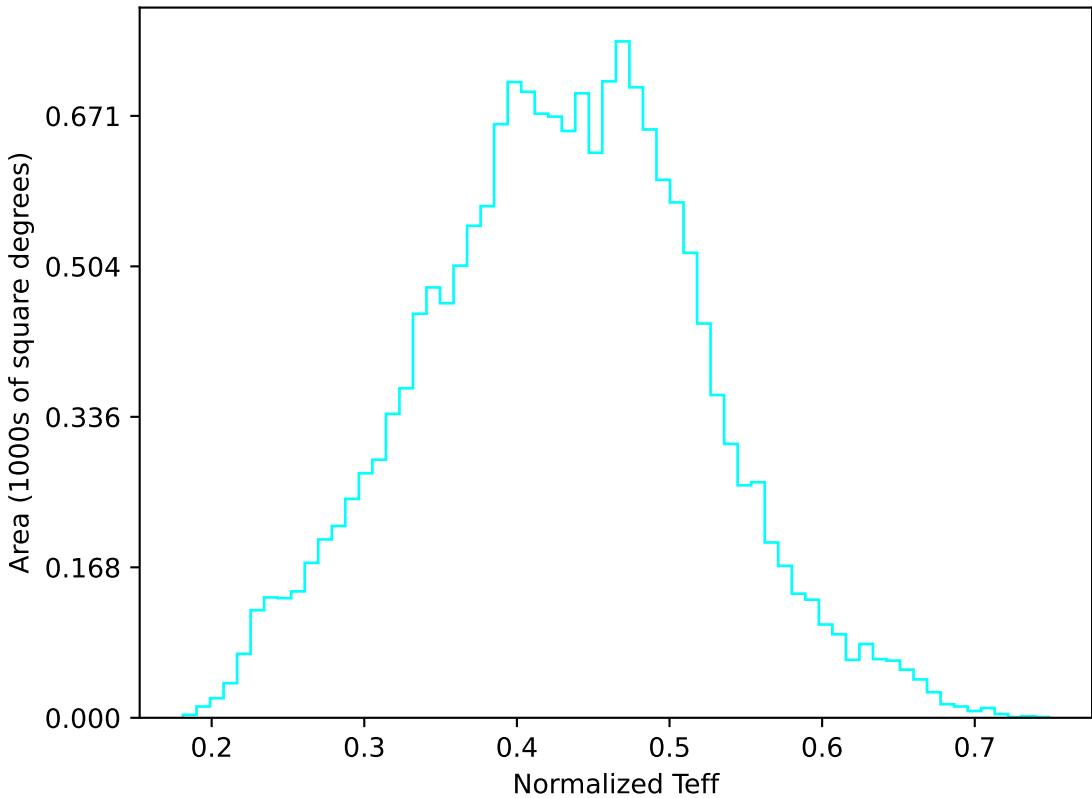
too_elab_r64_d2_ugrizy_v3.4_10yrs WFD u band: Normalized Teff
