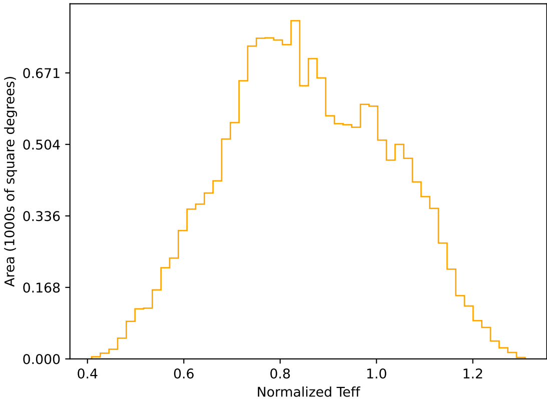
too_elab_r64_d2_ugrizy_v3.4_10yrs WFD r band: Normalized Teff
