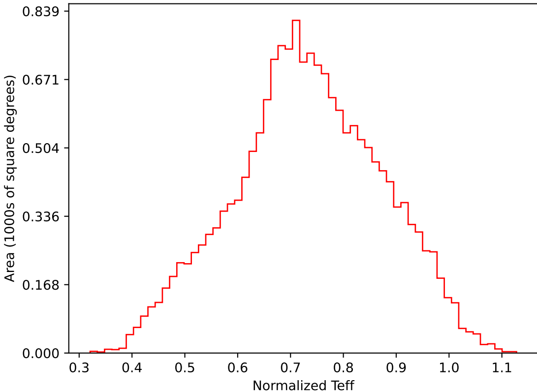
too_elab_r64_d2_ugrizy_v3.4_10yrs WFD i band: Normalized Teff
