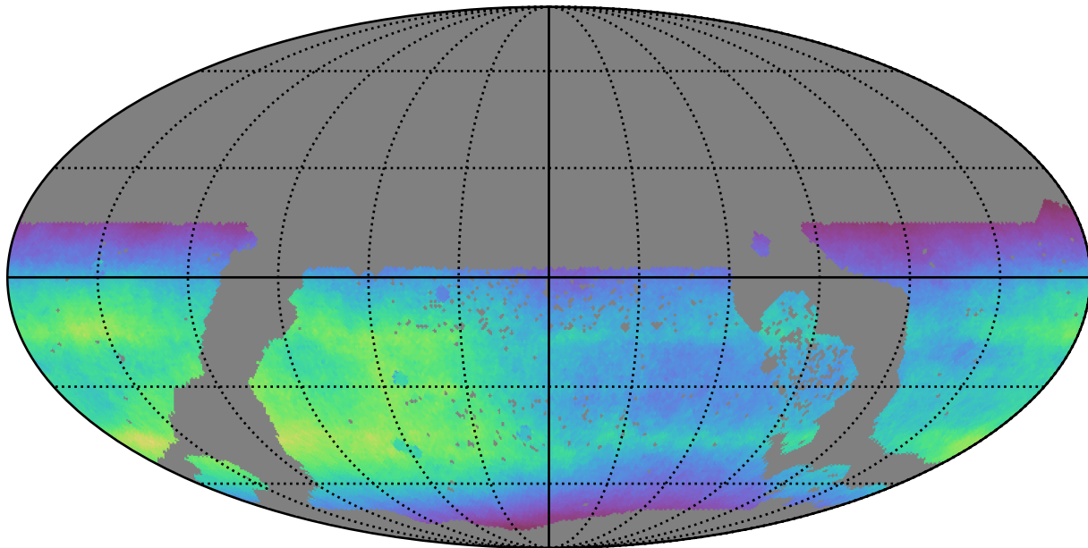
too_elab_r64_d2_ugrizy_v3.4_10yrs WFD all bands: Normalized Teff
