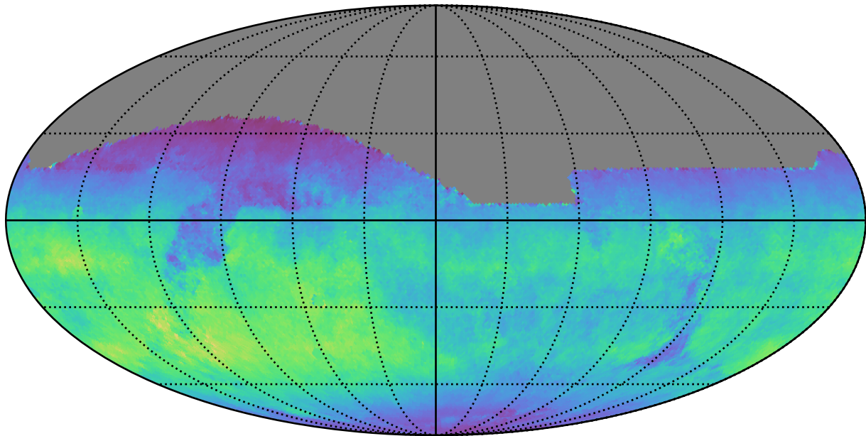
too_elab_r64_d2_ugrizy_v3.4_10yrs All sky z band: Normalized Teff
